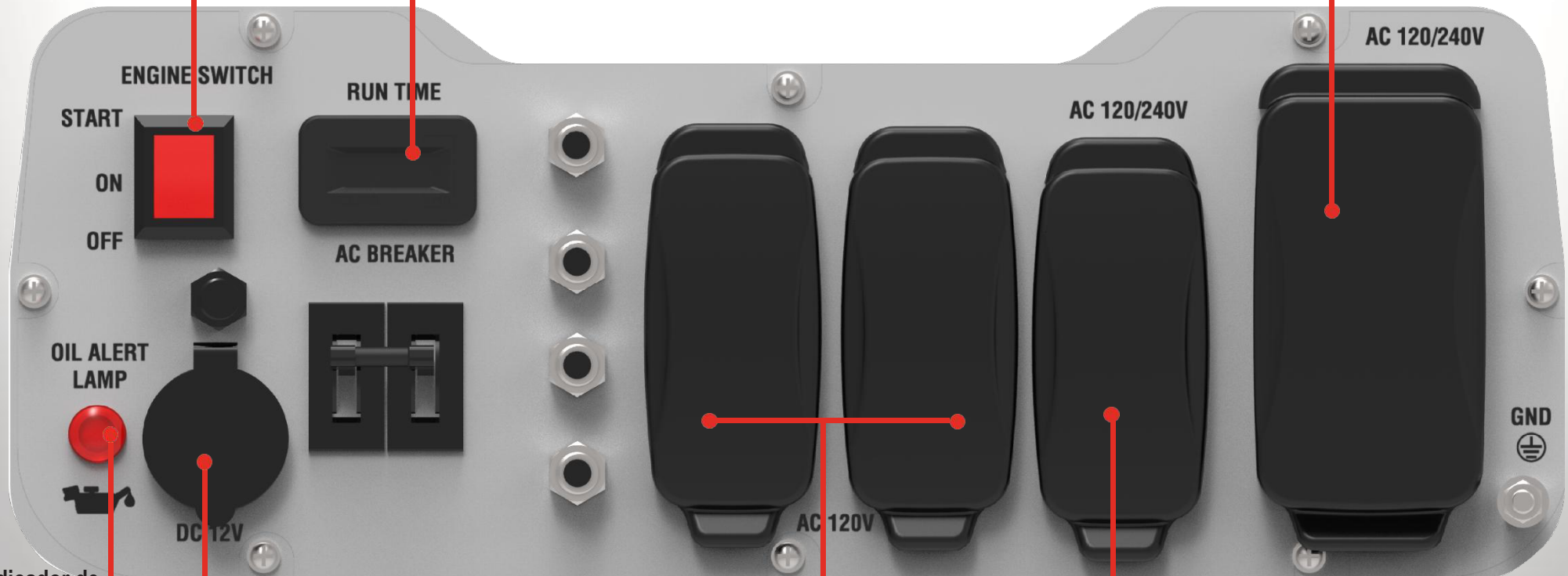
(1) 120/240V AC 30A L14-30R
